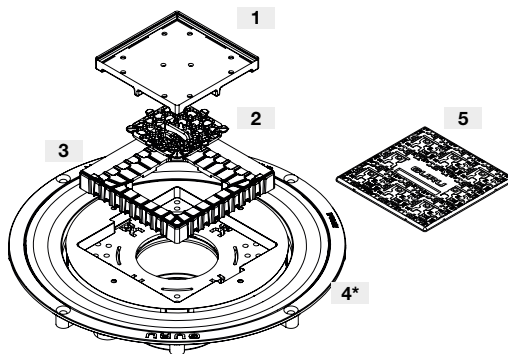
EVO GRATE INTEGRA 4" - under ¼"
