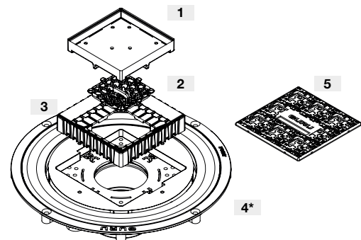
EVO GRATE INTEGRA 4" - over ¼"
